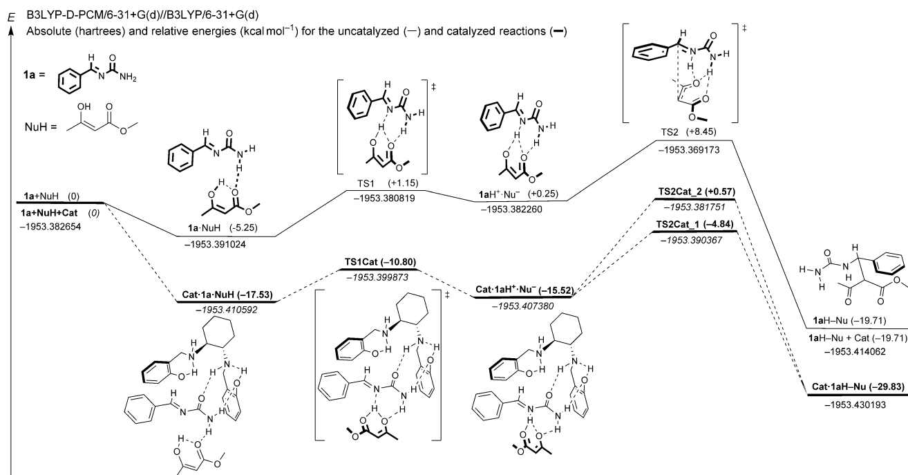
Figure 1. Absolute and relative free energies (B3LYP-D-PCM/6-31 + G*/B3LYP/6-31 + G*) of the species involved in the catalyzed (bold lines) and uncatalyzed reaction 1a + NuH (methyl acetoacetate, enol form).
